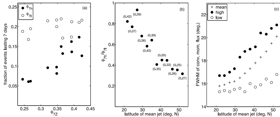
Figure 2. Results for 12 runs with varying stirring latitudes. (a) The frequency of high- ( \phi_{7h} ) and low-phase ( \phi_{7l} ) events persisting for at least 7 days versus the autocorrelation of the run's annular mode time series Z at a lag of 7 days ( \phi_{7Z} ). (b) The ratio of \phi_{7h} and \phi_{7l} versus the latitude of the mean jet, with \phi_{7Z} plotted adjacent to each point. (c) The full-width at half-maximum (FWHM) of the eddy forcing for the time mean and composites of the top (high) and bottom (low) 10% of annular mode events.
