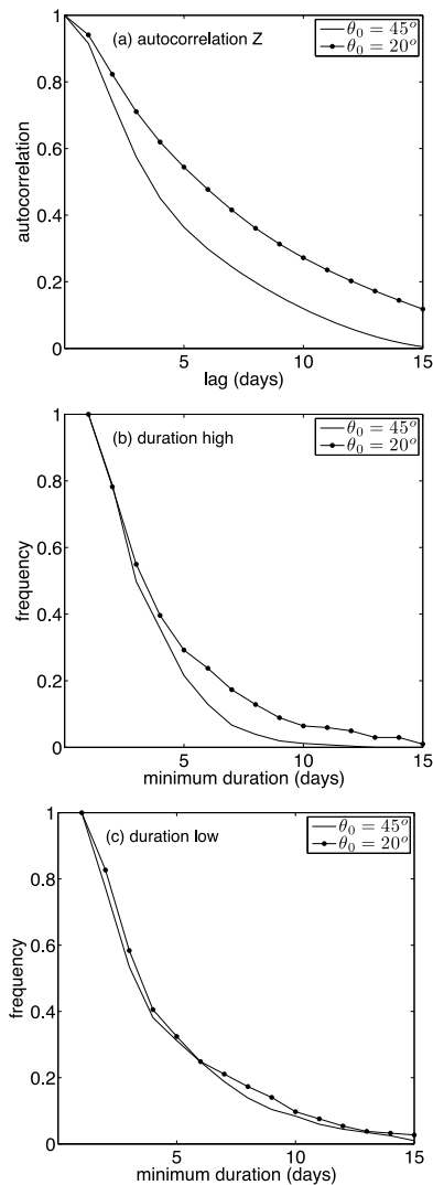
Figure 1. (a) The autocorrelation of the annular mode time series Z for two runs of varying stirring latitude \theta_0 . (b and c) Frequency of high- and low-phase events that persist for at least a certain number of days, where a high- (low-) phase event is defined for values in the top (bottom) 10% of Z .
