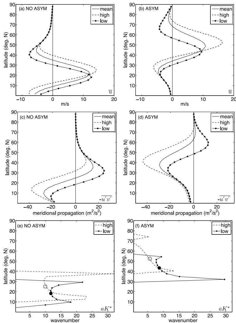
Figure 3. Results for the NO ASYM and ASYM free model runs, where the high- and low-phase are composites defined by the top and bottom 10% of the annular mode index Z . (a and b) Zonal-mean zonal wind profiles and (c and d) the meridional propagation of the eddies defined by the zonally averaged meridional flux of zonal momentum ( -u'v' ). Positive (negative) values imply poleward (equatorward) wave propagation. (e, f) K^* defined in (3) times the radius of the earth a for the high- and low-phase zonal wind profiles averaged over phase speeds 0–4 m/s. The large open (filled) circle denotes the position of the high- (low-) phase jet where the calculation was centered.
